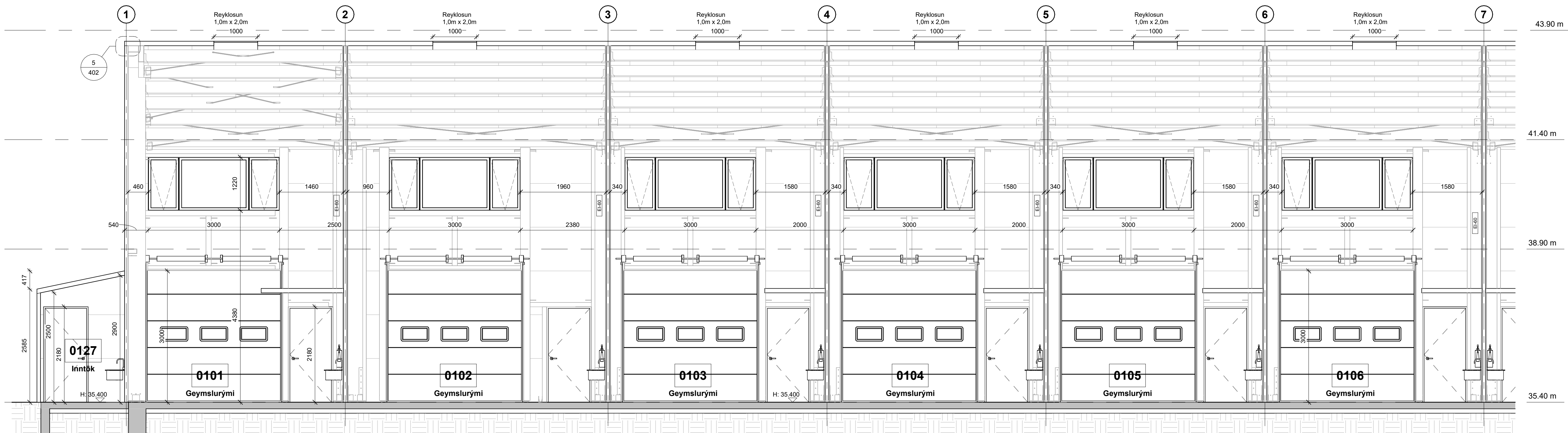
SNID C - Hluti 1-7 1 : 50
